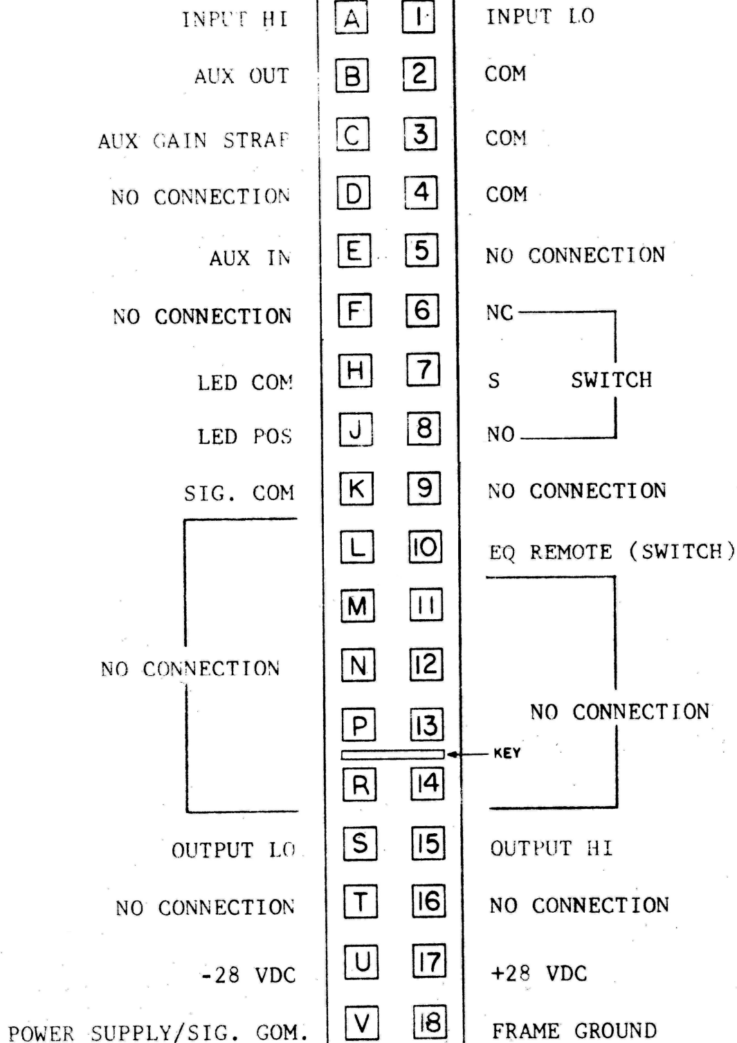
TERMINAL VIEW OF RECEPTACLE
