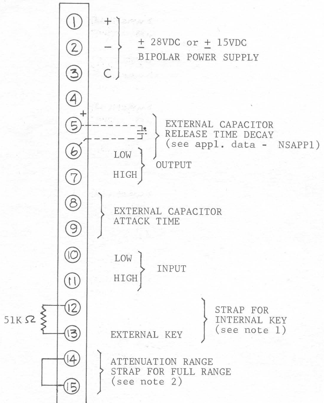
TERMINAL VIEW OF RECEPTACLE
